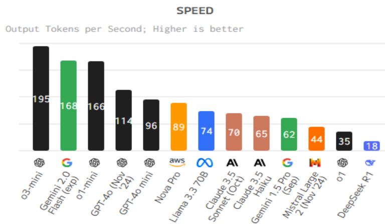
Artificial Analysis Index (Speed)
