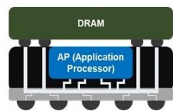
InFO-PoP Structure
