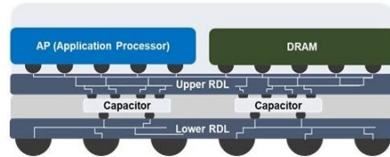
WMCM Structure
