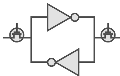
SRAM Cell
